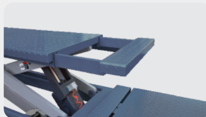
Extendable varying platform suitable for varying wheelbases.
