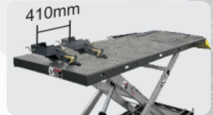
Front Wheel Vise positioning Front wheel distance vise with of an 410mm.
